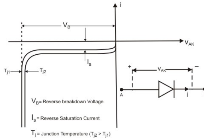
Fig 2.5: Reverse bias i-v characteristics of a power Diode.
