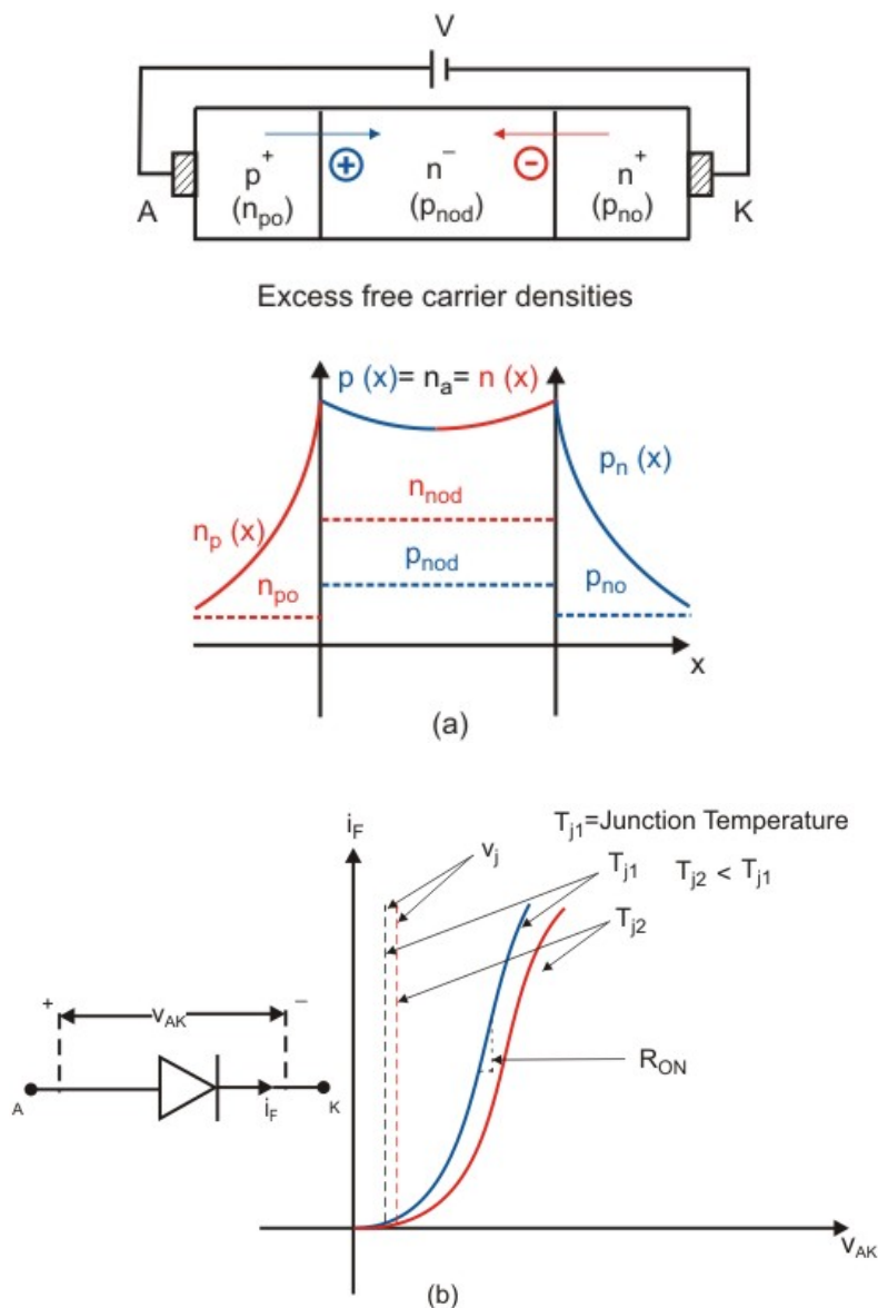
Fig 2.7: Characteristics of a forward biased power Diode; (a) Excess free carrier density distribution; (b) i-v characteristics.
