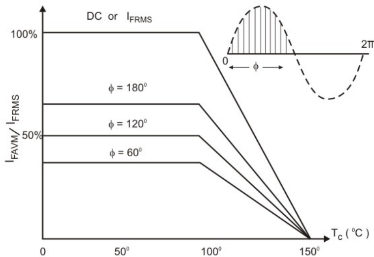
Fig 2.8: Derating curves for the forward current of a Power Diode.
