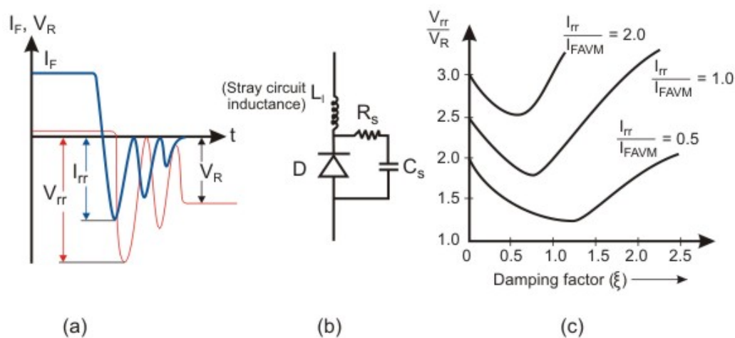
Fig. 2.14: Diode overvoltage protection circuit; (a) “Snappy recovery characteristics; (b) Capacitive snubber circuit; (c) snubber characteristics.
