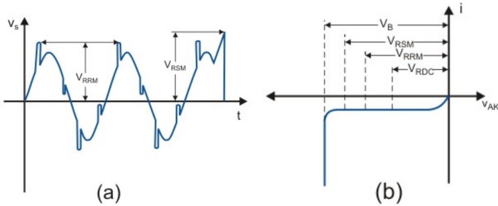
Fig. 2.6: Reverse Voltage ratings of a power diode; (a) Supply voltage wave form; (b) Reverse i-v characteristics
