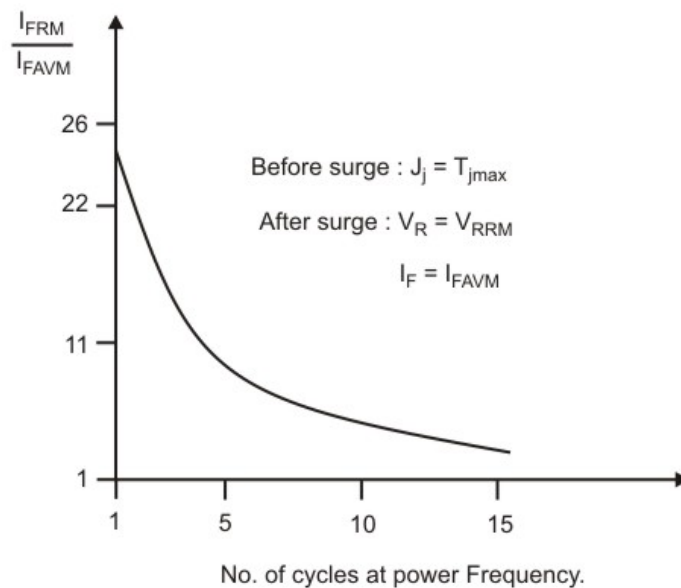
Fig 2.10: Peak Repetitive surge current VS time curve of a power diode.
