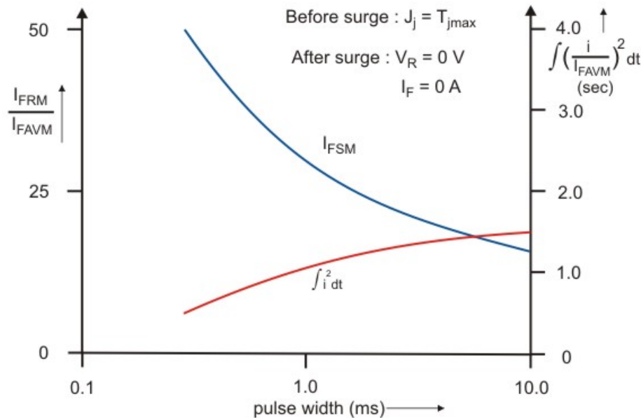
Fig. 2.11: Non-repetitive surge current and surge current integral vs. current pulse width characteristics of a power Diode.
