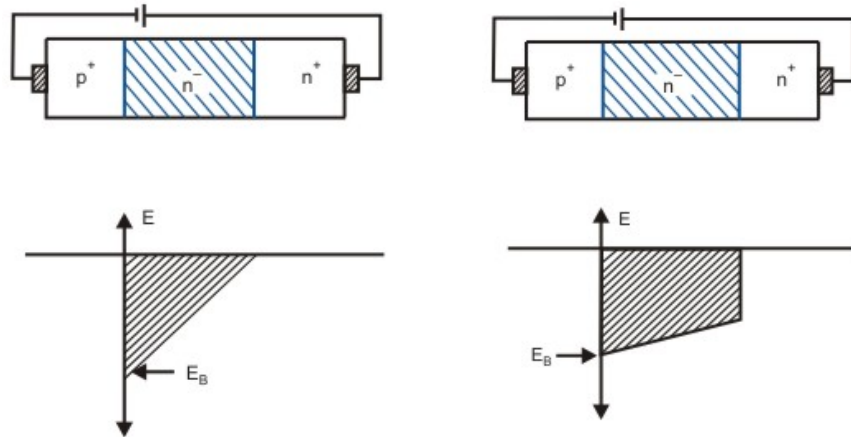
Fig 2.4: Electric field strength in reverse biased power Diodes; (a) Non-punch through type; (b) punch through type.
