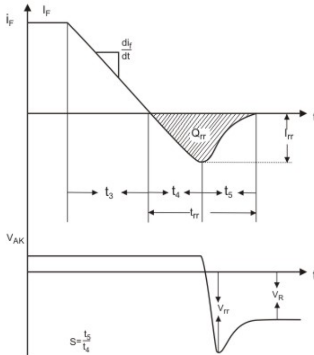
Fig. 2.13: Reverse Recovery characteristics of a power diode
