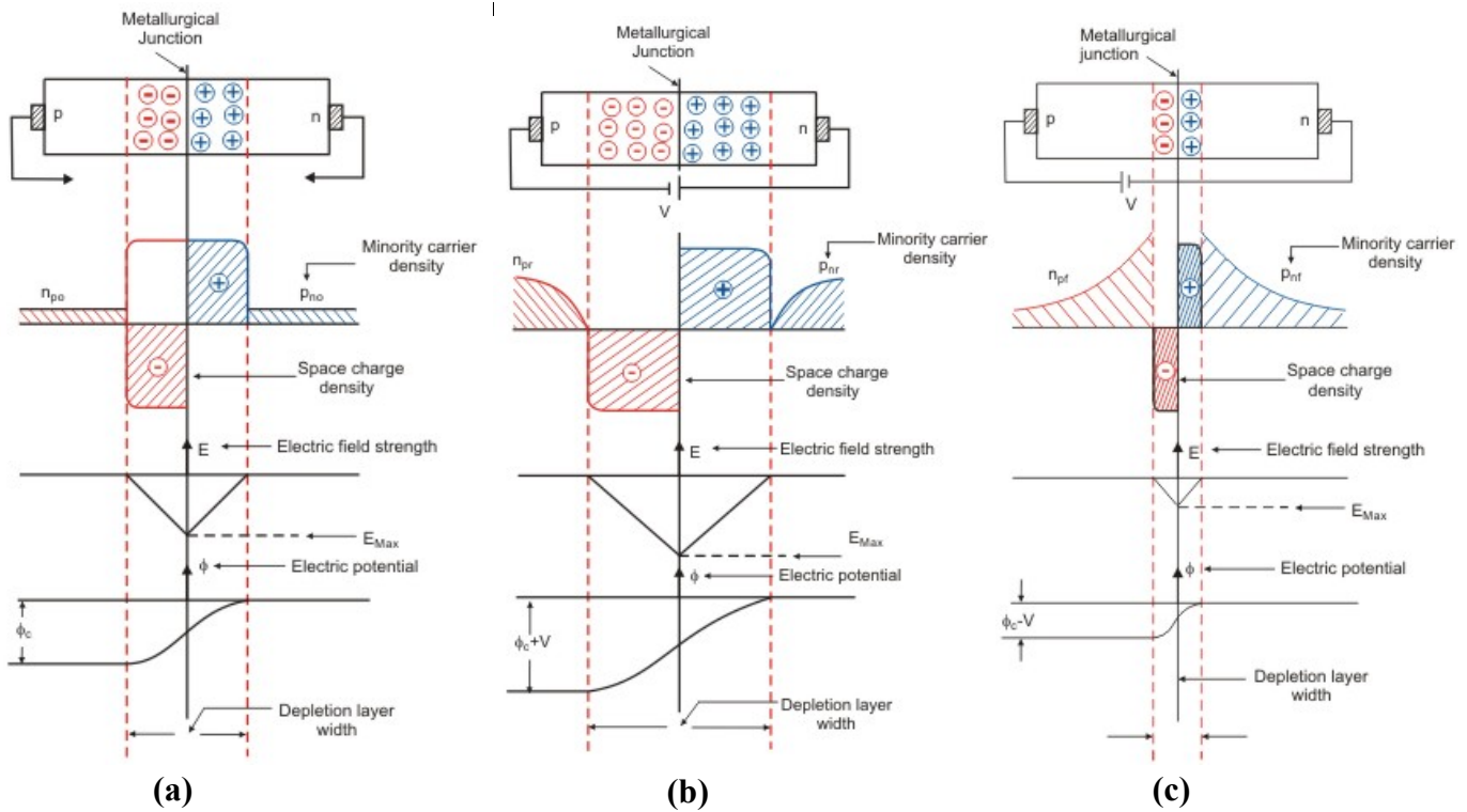
Fig 2.1: Space charge density the electric field and the electric potential in side a p-n junction under (a) thermal equilibrium condition, (b) reverse biased condition, (c) forward biased condition.
