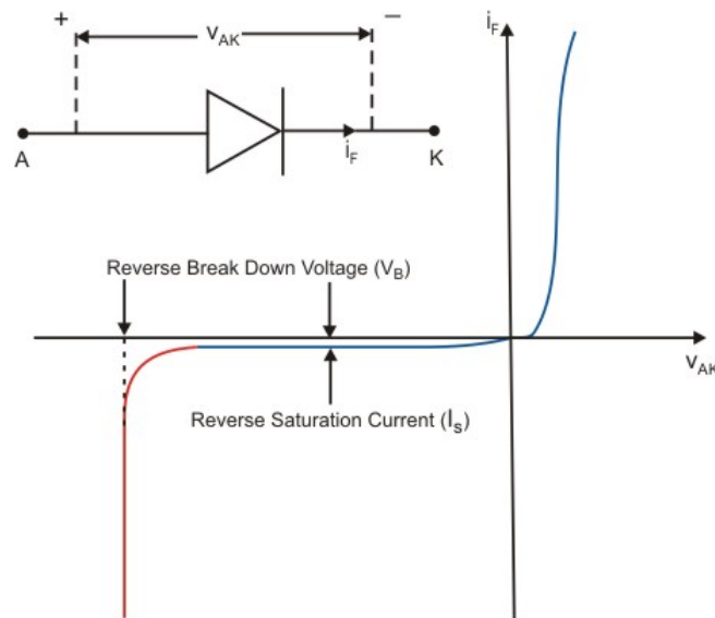
Fig 2.2: Volt-Ampere ( i-v ) characteristics of a p-n junction diode
