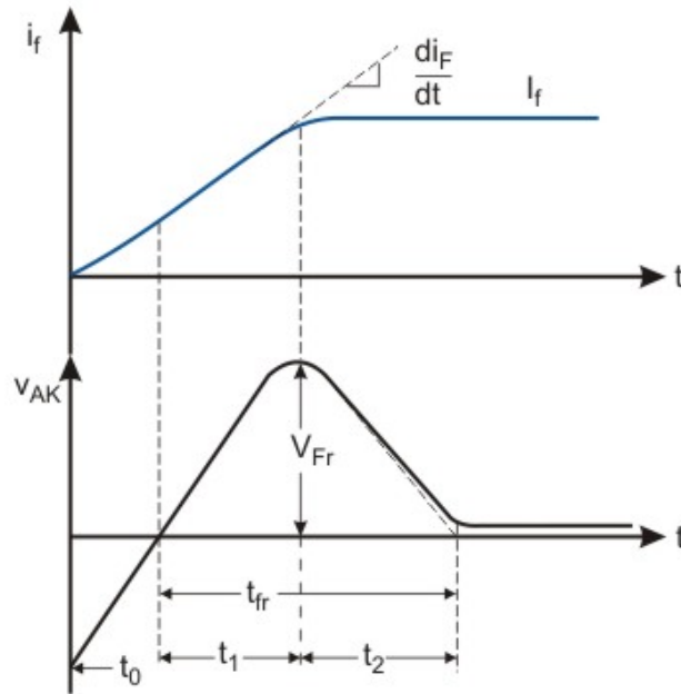
Fig. 2.12: Forward current and voltage waveforms of a power diode during Turn On operation.
