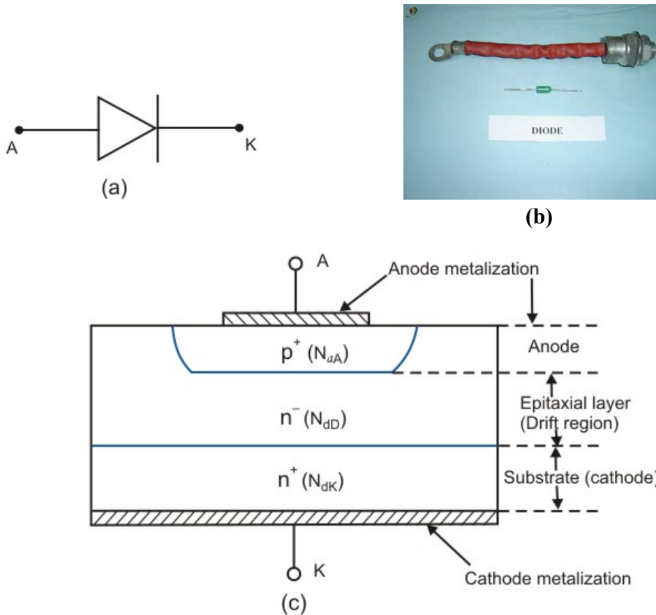
Fig. 2.3: Diagram of a power; (a) circuit symbol (b) photograph; (c) schematic cross section.
