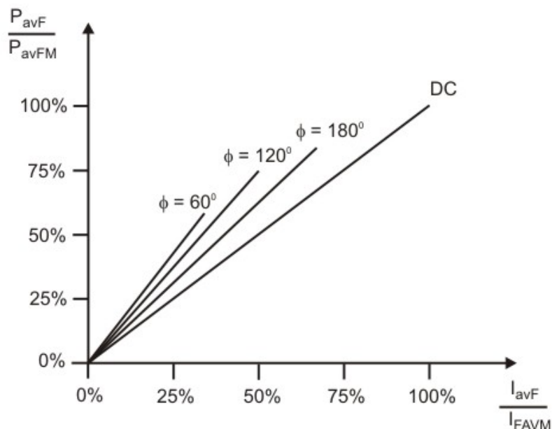
Fig 2.9: Average forward power loss vs. average forward current of a power Diode.
